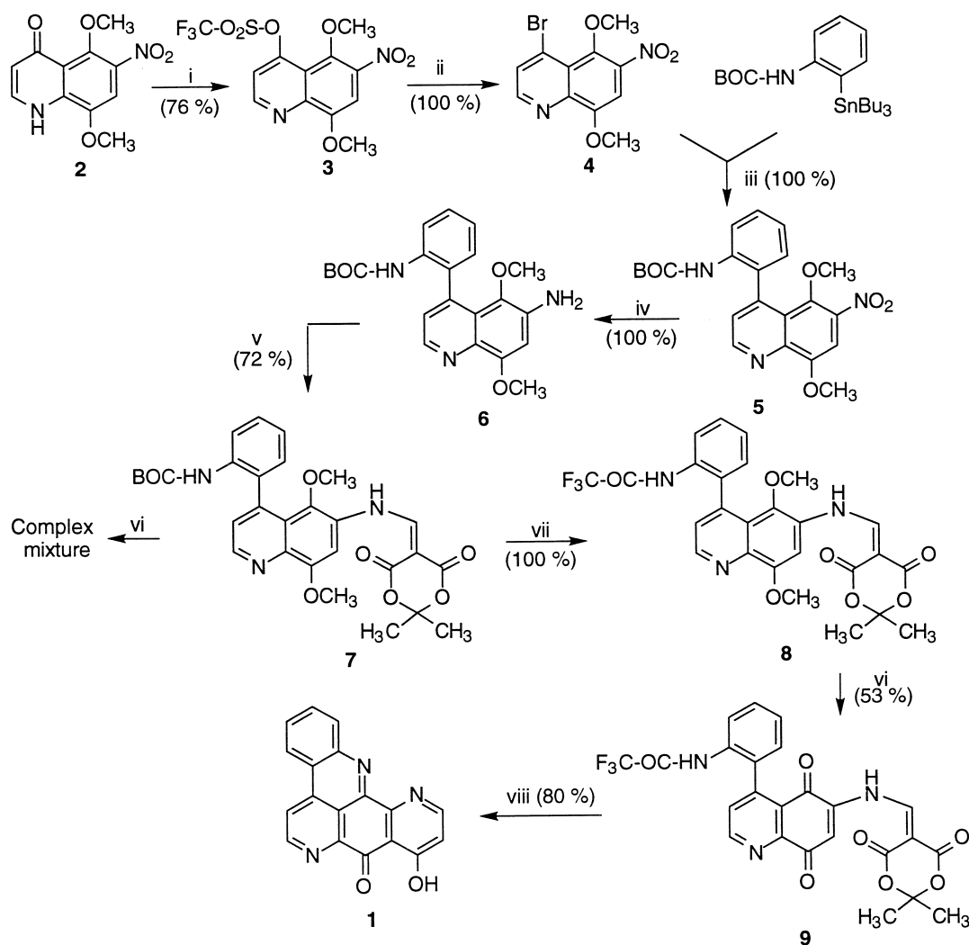
Scheme 2. Reagents and conditions: (i) \text{F}_3\text{C}-\text{O}_2\text{S}-\text{O} , 2,6-lutidine, DMAP, \text{CH}_2\text{Cl}_2 , rt, 20 h; (ii) LiBr, 1,4-dioxane, reflux, 2 h; (iii) \text{PdCl}_2(\text{CH}_3\text{CN})_2 , 1,4-dioxane, 55 °C, 14 h; (iv) Cyclohexene, Pd-C (10%), EtOH, reflux, 45 min; (v) Meldrum's acid, \text{HC}(\text{OEt})_3 , reflux, 2 h, then add 6 , reflux, 4 h; (vi) (\text{NH}_4)_2\text{Ce}(\text{NO}_3)_6 , \text{CH}_3\text{CN} , 2 M \text{H}_2\text{SO}_4 , rt, 3 h; (vii) TFA, TFAA, rt, 90 min; (viii). \text{Ph}_2\text{O} , 200–220 °C, 15 min.
