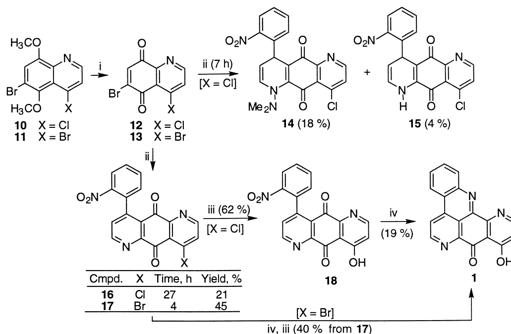
Scheme 3. Reagents and conditions: (i) (\text{NH}_4)_2\text{Ce}(\text{NO}_3)_6 , \text{CH}_3\text{CN} , \text{H}_2\text{O} , 0^\circ\text{C} , 3 h; (ii) o -Nitrocinnamaldehyde dimethylhydrazone (neat), ultrasound, 50^\circ\text{C} ; (iii) \text{CF}_3\text{CO}_2\text{H}\cdot\text{CHCl}_3 (3:1), rt, 5 min; (iv) \text{H}_2 , Pd-C, 1 atm, 1 h.
